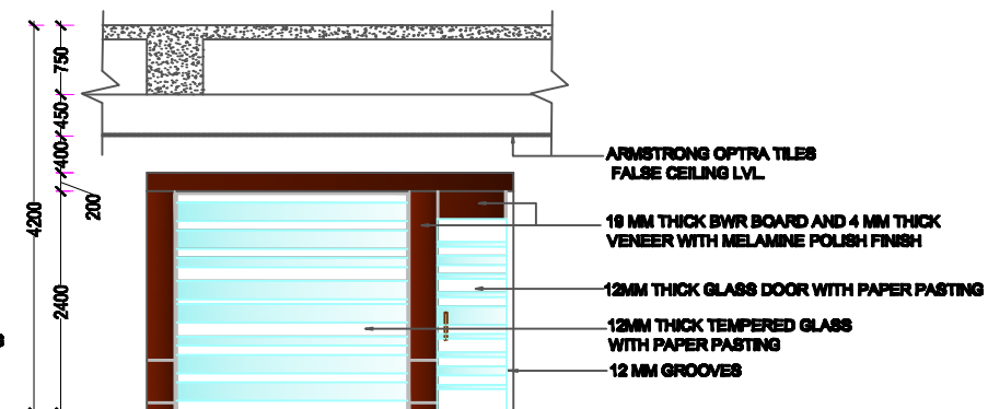
ELEVATION F
