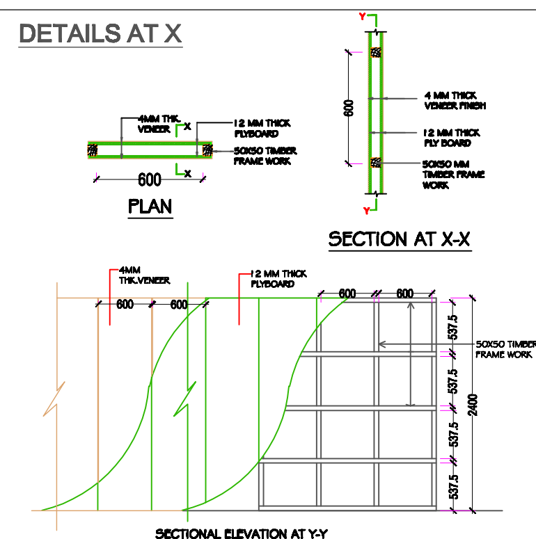
SECTIONAL ELEVATION AT Y-Y
