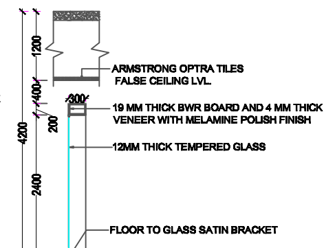
SECTION 2-2
